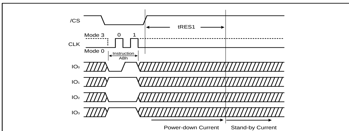
Figure 34b. Release Power-down Instruction (QPI Mode)
